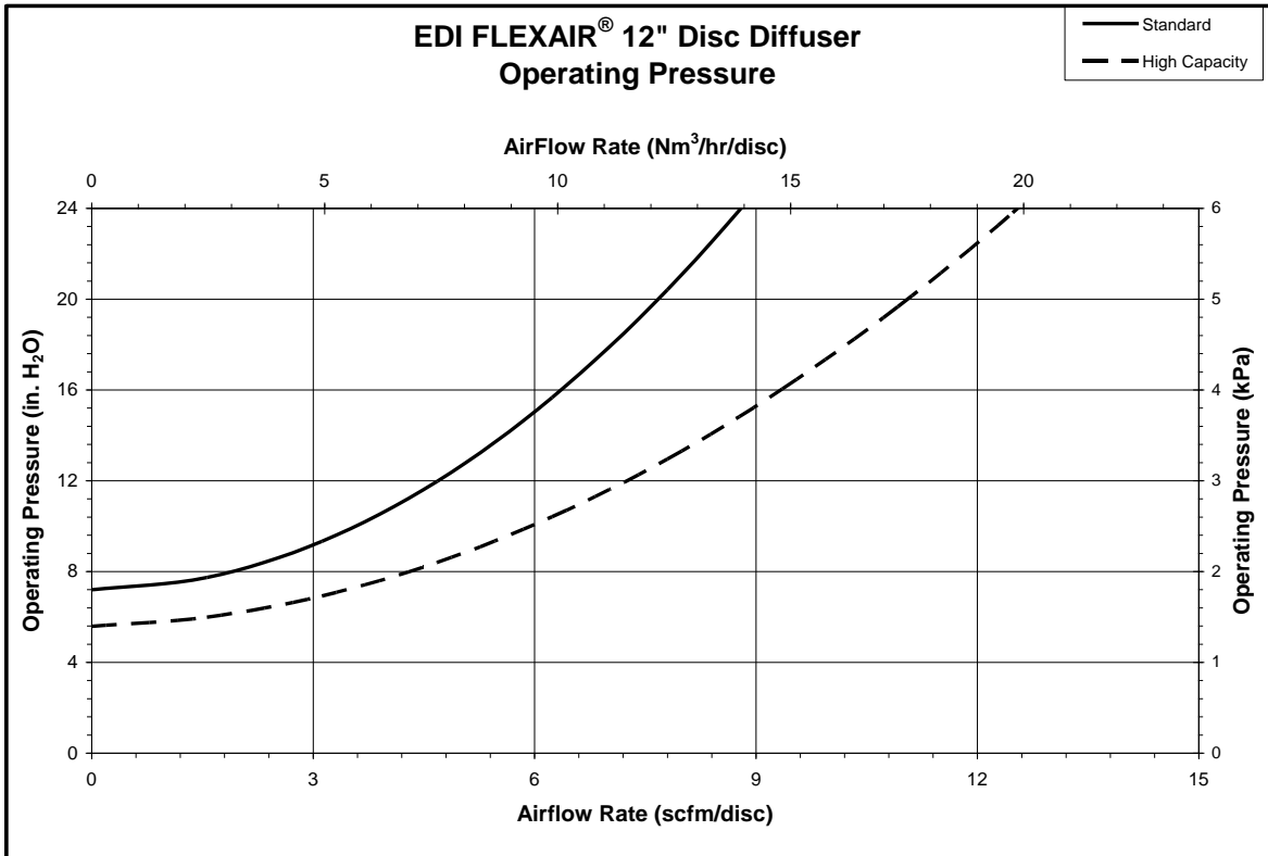
12" Disc utilizes a 13/32" orifice with Standard perforation and 7/8" orifice with High Capacity perforation.
