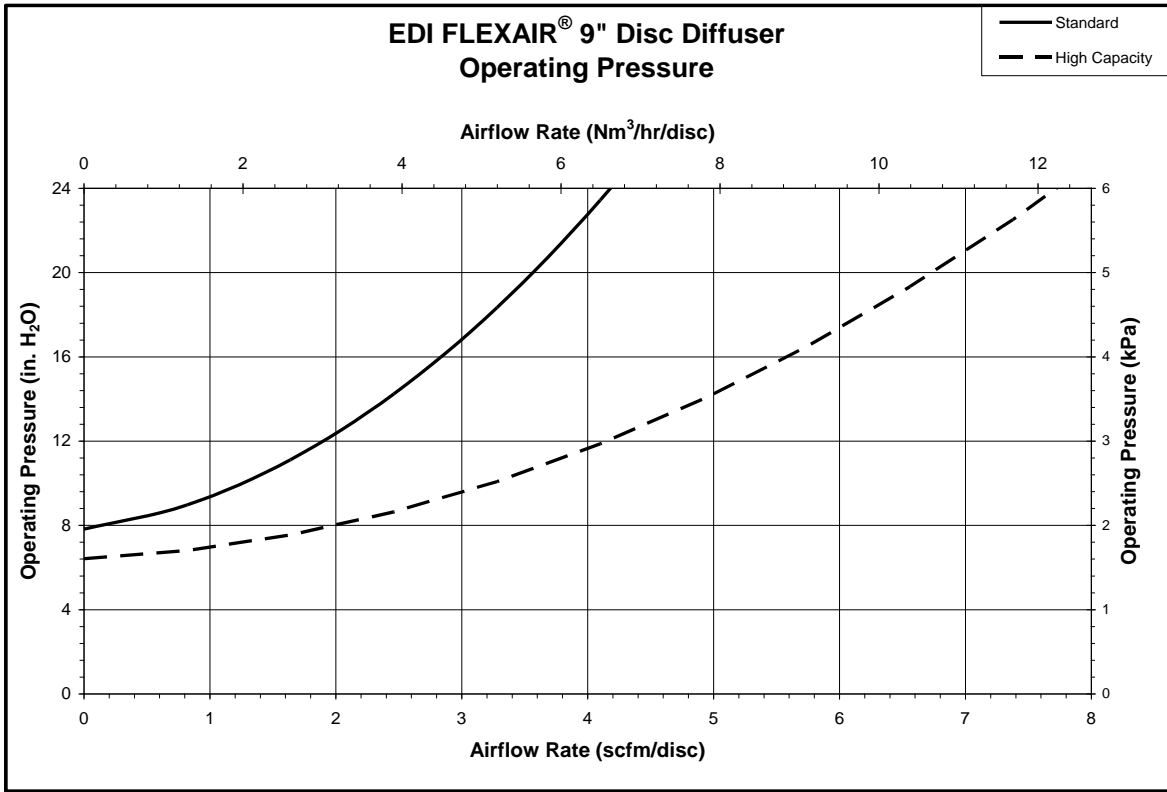
9" Disc utilizes a 1/4" orifice with Standard perforation and 3/8" orifice with High Capacity perforation.
